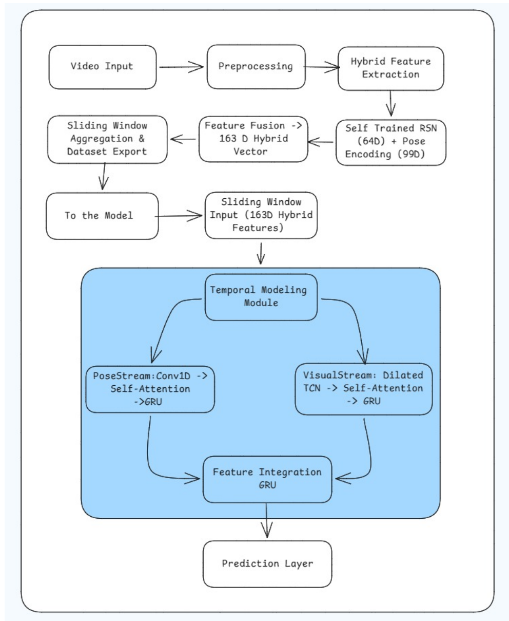
Fig. 1 Smashifix Dual-Pipeline Architecture
