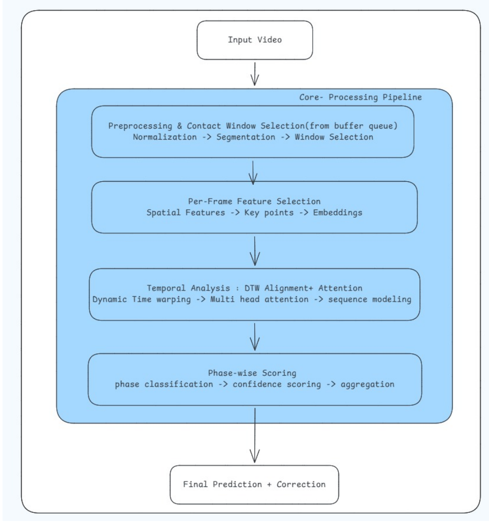
Fig. 3 Detailed Prediction Pipeline
