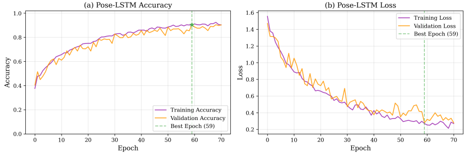
Fig. 7 Pose-LSTM Training Curves
