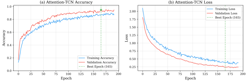
Fig. 6 Attention-TCN Training Curves
